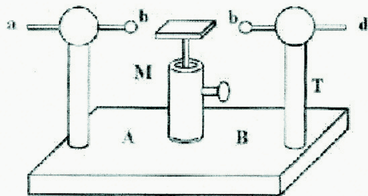
Figure 3 The apparatus described by Izarn in 1804. Author's reconstruction of IZARN (1804), fig. 53, plate III, facing p. 130.
