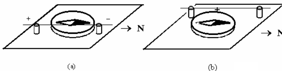
Fig. 4 – During the lecture experiment Ørsted attempted to observe the magnetic effect of the electric current following his second hypothesis. If he put the conducting wire above the magnetic needle (as stated by Ørsted) he should choose a position slightly to the East (a) or the the West (b) because he expected that one of the poles would be attracted and the other would be repelled by the wire. He would expect the magnetic needle to turn in opposite directions in the situations (a) and (b). However, according to current knowledge, we know that the needle would always turn to the same side in both cases. Ørsted would be unable to understand the result of this experiment, according to his first or second hypotheses.
