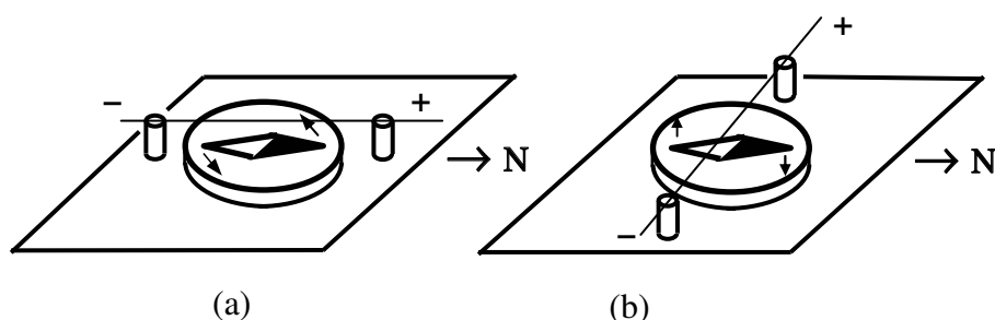
Fig. 2 – (a) “Ørsted’s experiment” as described in textbooks: the conducting wire is placed over the magnetic needle, in the North-South direction; when the electric current passes through the wire, the magnetic needle turns as shown by the arrows. (b) Ørsted’s early experiments: the wire is placed over the magnetic needle, in the East-West direction; he expected the magnetic poles to be impelled parallel to the wire in opposite directions, producing a rotation of the magnetic needle, but observed no effect. In this position, according to current knowledge, the magnetic needle suffers a deflection in the vertical plane which is difficult to observe.
